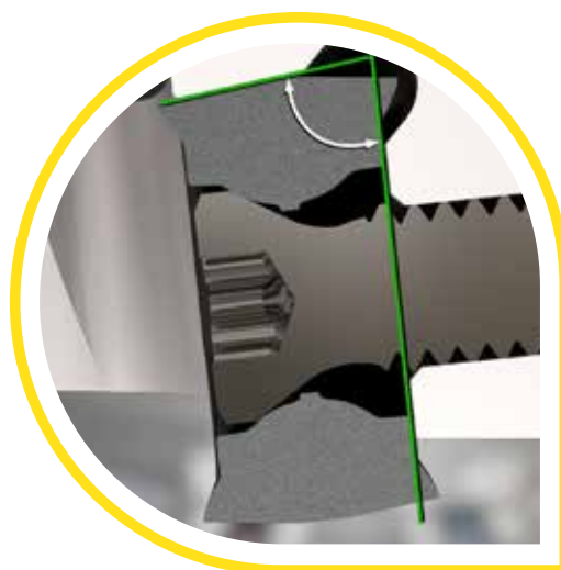
Dovetail Insert Pocket Locks the Insert Firmly in Place
